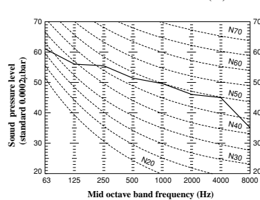
Models FDC508HES3 FDCP508HES3 Noise level 55 dB (A)
