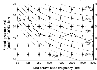
Models FDC408HES3 FDCP408HES3 Noise level 54 dB (A)
