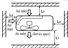
Models FDC(P)208~508 type
