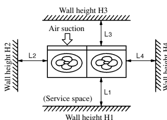
Models FDC808, 1008 type
