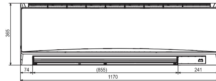
Front View
