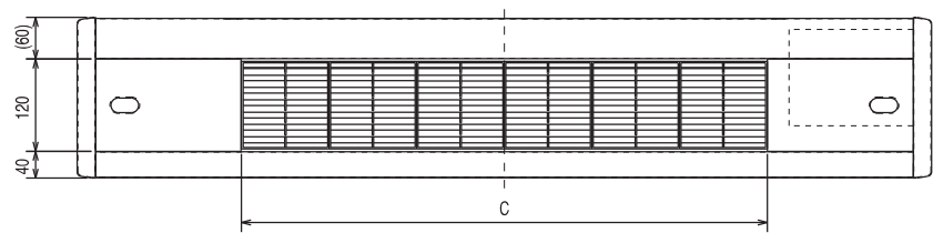
Upper View
