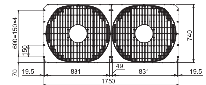
Upper View
