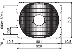
Upper View
