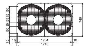
Upper View
