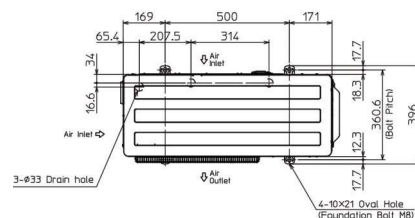
Upper View
