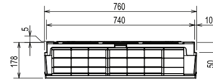
Upper View
