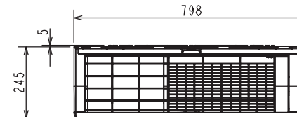
Upper View
