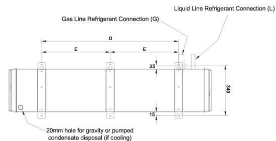
Upper View
